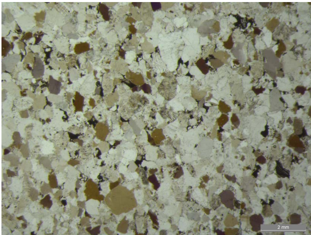
Figure 2 - Photomicrograph of Birchover Gritstone under Plane Polarised Light
