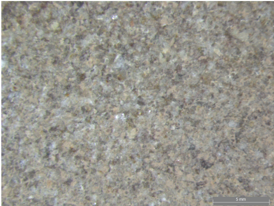
Figure 1 - Photomicrograph of Birchover Gritstone under Stereomicroscope
