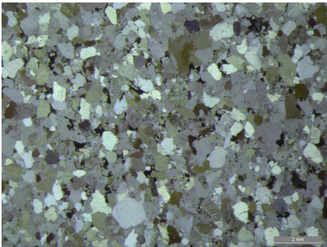
Figure 3 - Photomicrograph of Birchover Gritstone under Stereomicroscope. Note homogenous distribution and well sorted grains.
